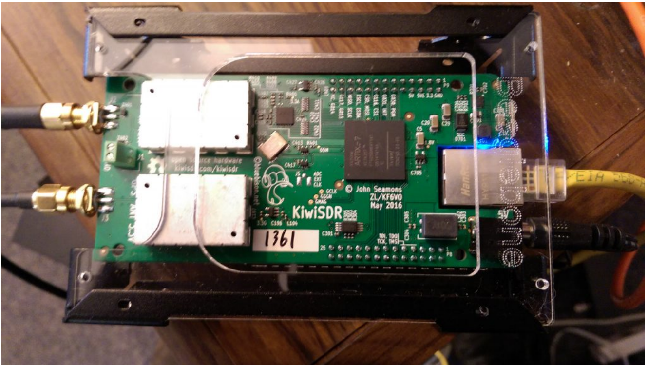
KiwiSDR kit assembled and in service.
